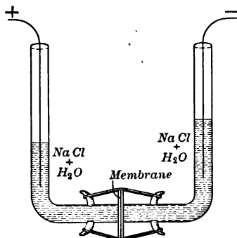
Effect of current on solution in tube.
